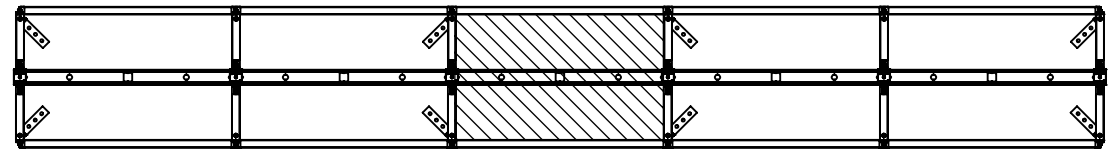
SIX UPRIGHTS REQUIRE EIGHT ANCHORS
