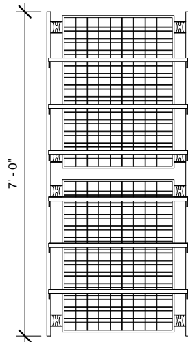
FRONT ELEVATION
